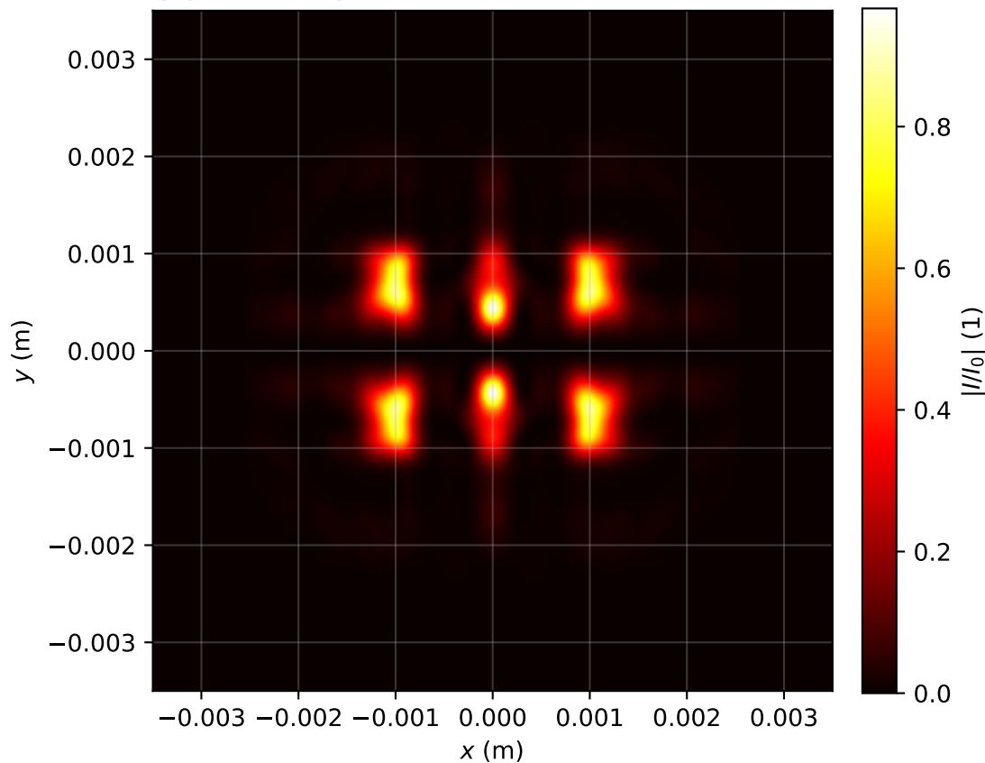
Intensity profile I(x, y, z = 1.911)/I_0 , P_{in}=6.0P_{cr} , artificial time
